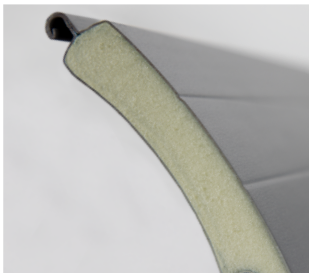
CFC-free foam within the aluminium lath provides thermal and acoustic insulation.
